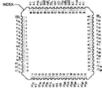
64 PIN VQFP (top view)
