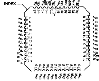
48 PIN PLCC (top view)
