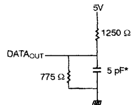
Figure 2. Output load.
